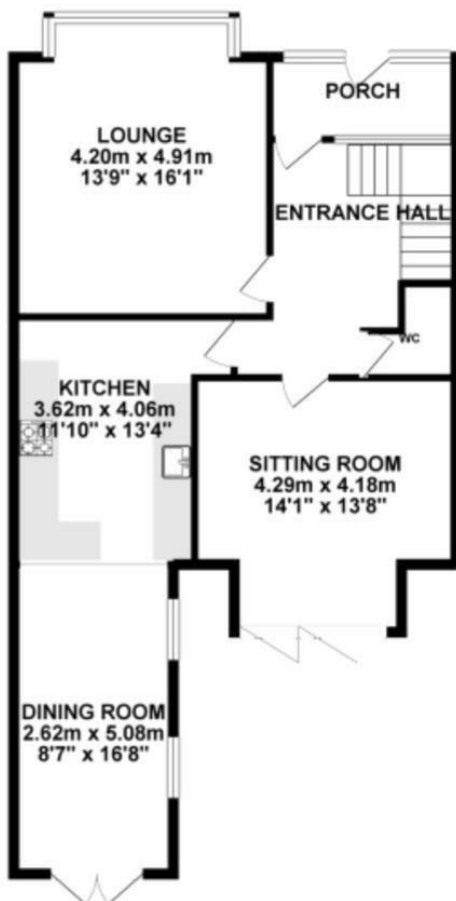
GROUND FLOOR 97.32 sq. m. ( 1047.58 sq. ft. )
